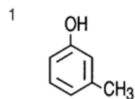
m -Cresol
