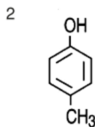
p -Cresol
