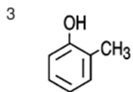
o -Cresol
