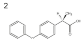
Fenoprofen (MW 242.3)
