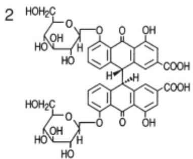
Sennoside A
