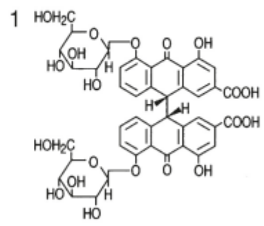
Sennoside B
